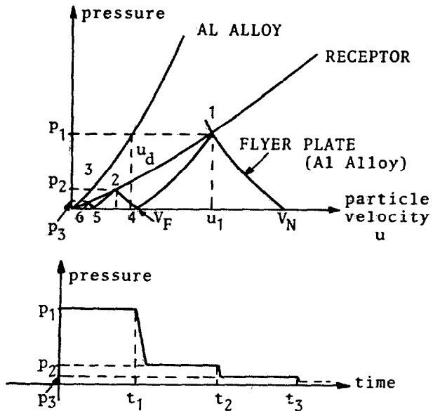
Fig 10 Principle of Generation of Rectangular Pressure Pulses
